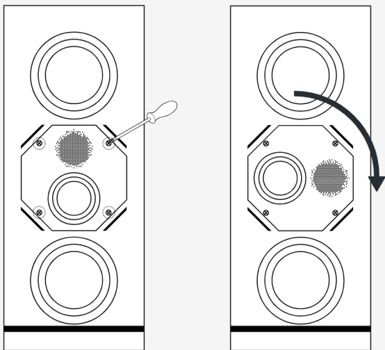
Unscrew holding screws
