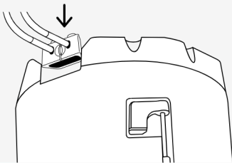
Attach Quik-Link to terminal panel
