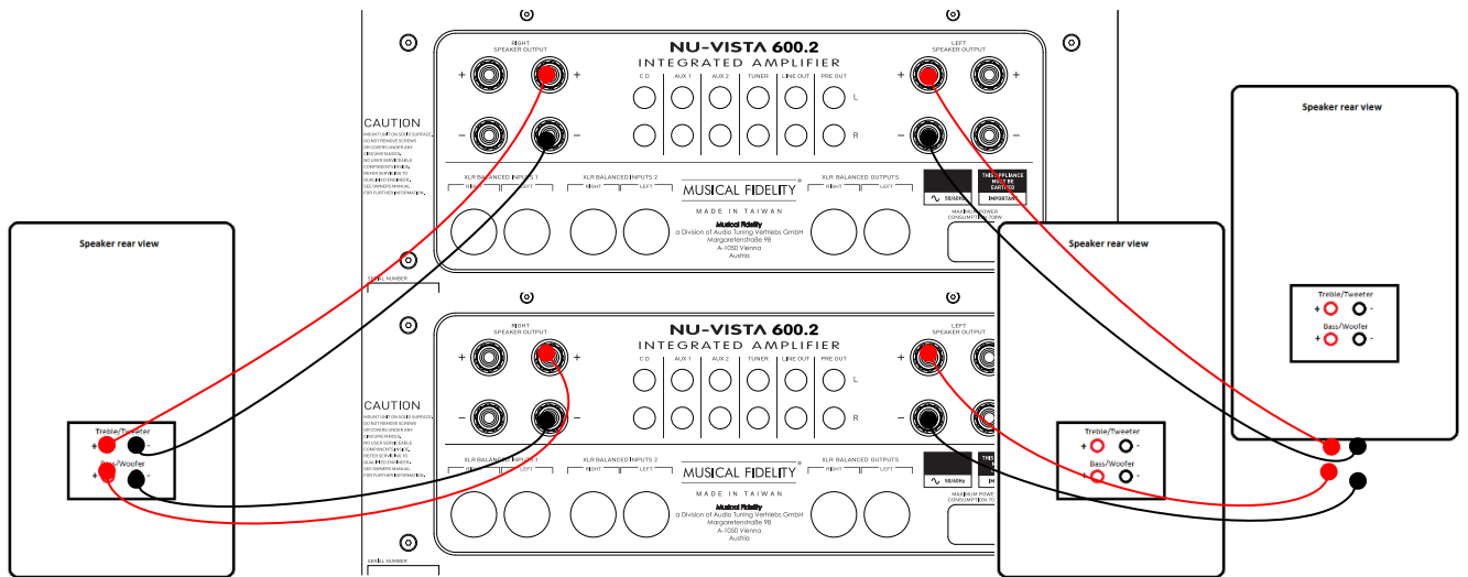
Bass/treble terminal links removed
