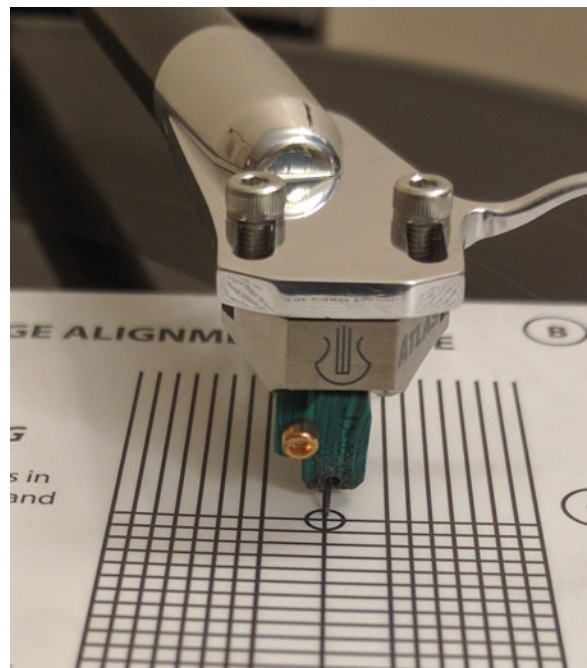
CENTRE LINE OF ALIGNMENT GAUGE
