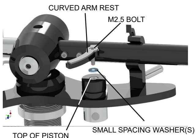
Diagram showing small spacing washers which set height of curved rest
